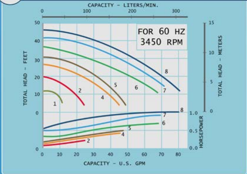
60HZ Lift Station Pump Curve for Part Number Configurator
